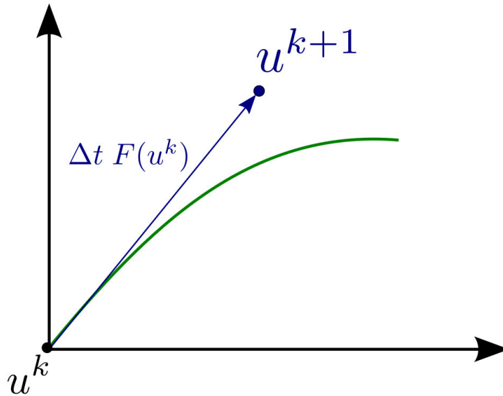
Explicit Euler
